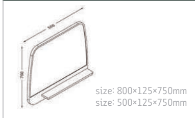
SWF-1500090M mirror in aluminium
